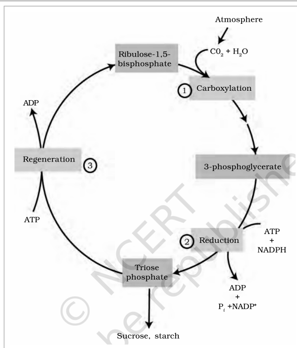
Fig. 11.8 - The Calvin cycle proceeds in three stages: (1) carboxylation , during which CO_2 combines with ribulose-1,5-bisphosphate; (2) reduction , during which carbohydrate is formed at the expense of the photochemically made ATP and NADPH; and (3) regeneration during which the CO_2 acceptor ribulose-1,5-bisphosphate is formed again so that the cycle continues.
