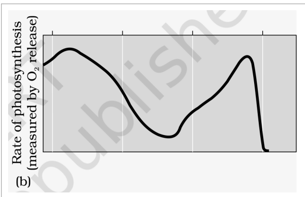
Fig. 11.3b - Graph showing the action spectrum of photosynthesis . Its vertical axis is Rate of photosynthesis (measured by O 2 release) . Panel marker: (b).
