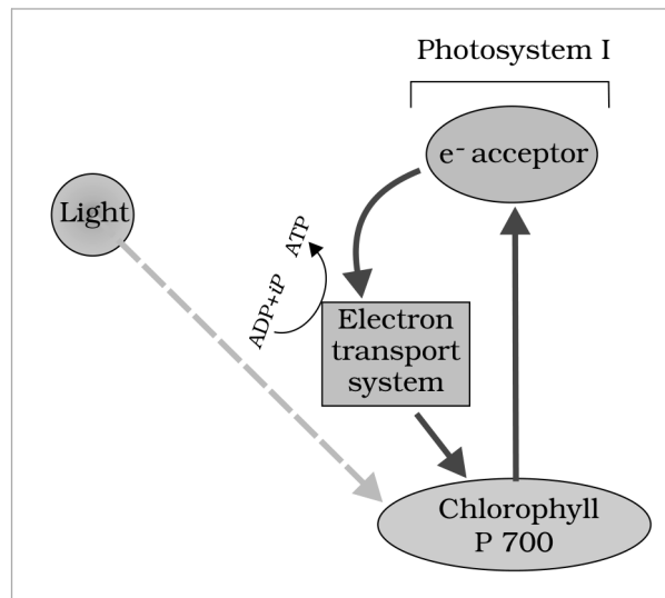
Fig. 11.6 - Cyclic photophosphorylation.
